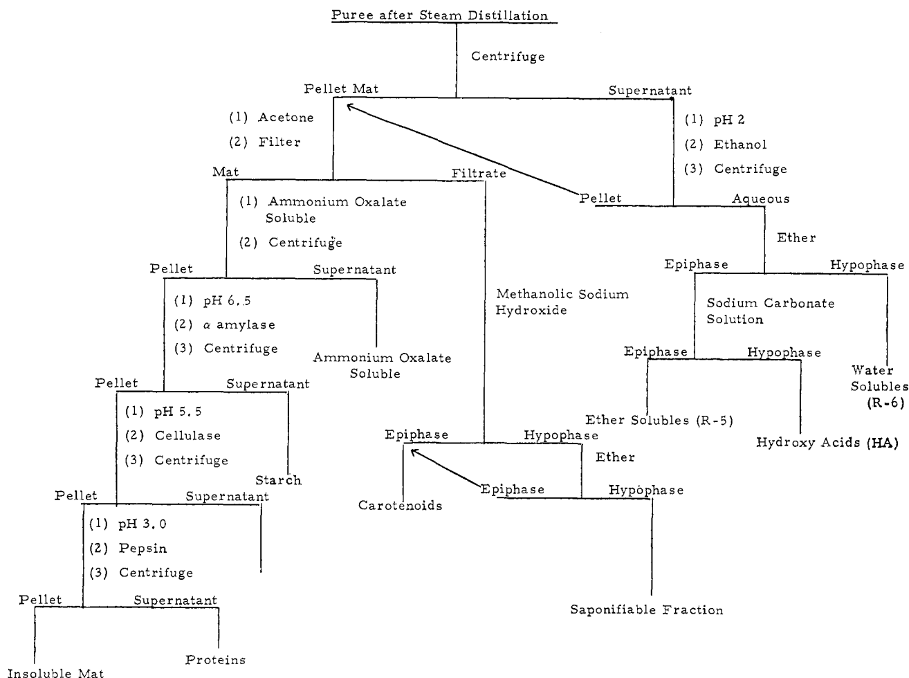
Figure 1. Flow sheet for fractionation of puree after steam distillation of dehydrated sweet potato flakes
